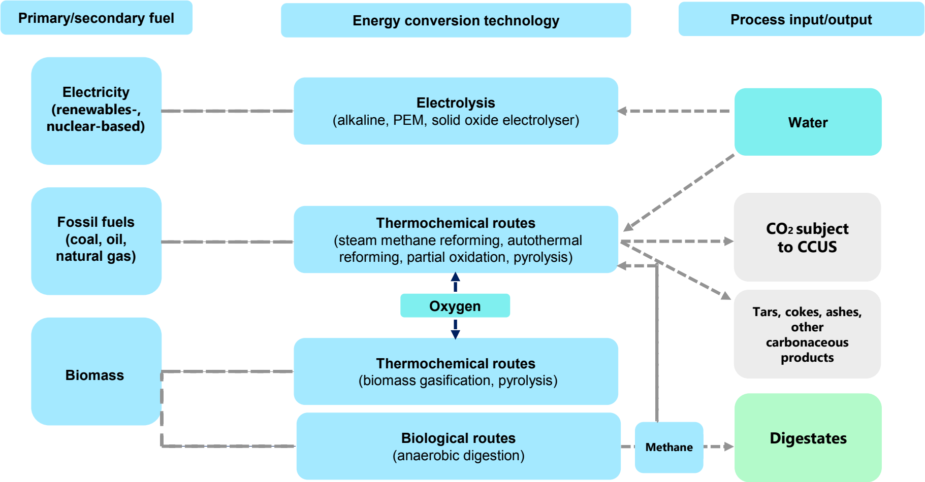
Simplified scheme of selected low-emissions hydrogen production routes
