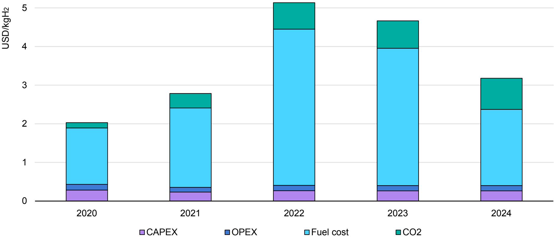
Estimated levelised cost of gas-based hydrogen produced via SMR without CCUS, 2020-2024
