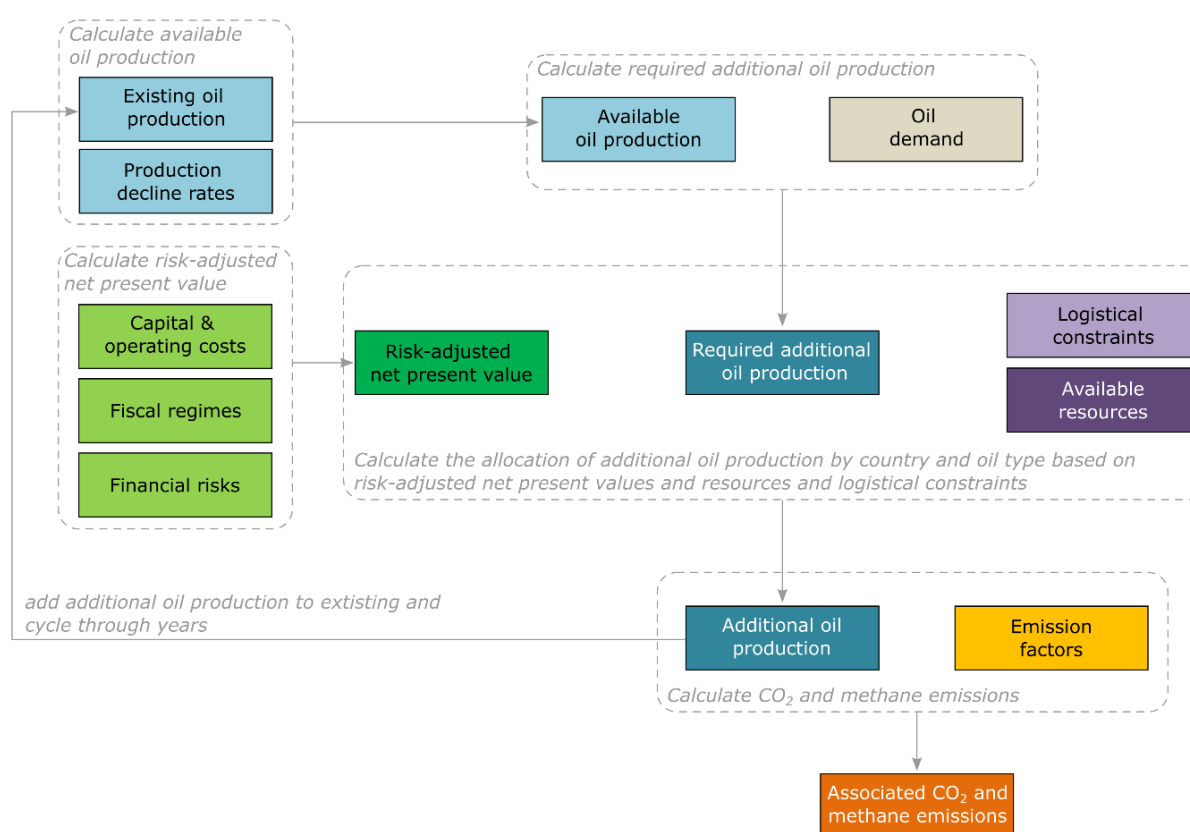
Figure 6.1 ▶ Structure of the oil supply module
