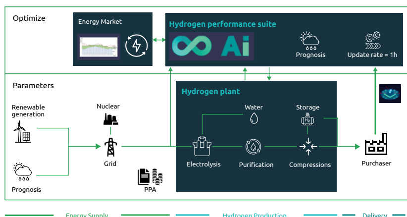
Figure. 17 - Hydrogen performance suite: balancing consumption, cost, and climate goals
