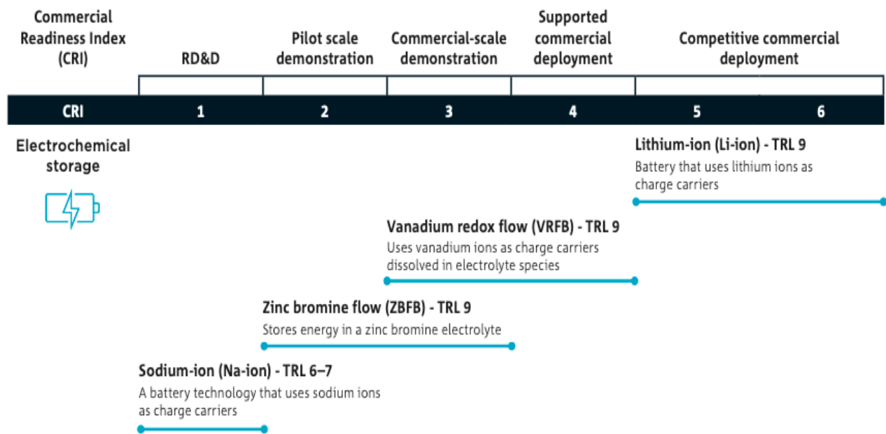
Figure 6-6 Assessment of Electrochemical Energy Storage Technology
