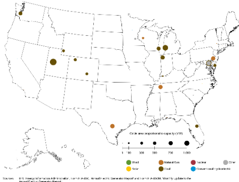
Figure 6.1.D. Utility-Scale Generating Units Planned to Retire from January 2025 to December 2025
