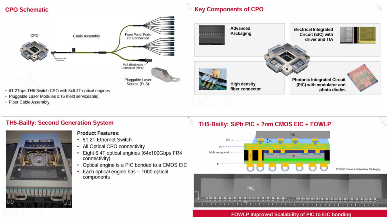
图58: TH5-Bailly 采用 SiPh PIC + 7nm CMOS EIC + FOWLP 架构
