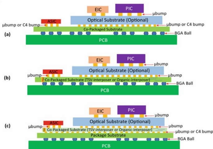
2D heterogeneous integration ASIC+PE
