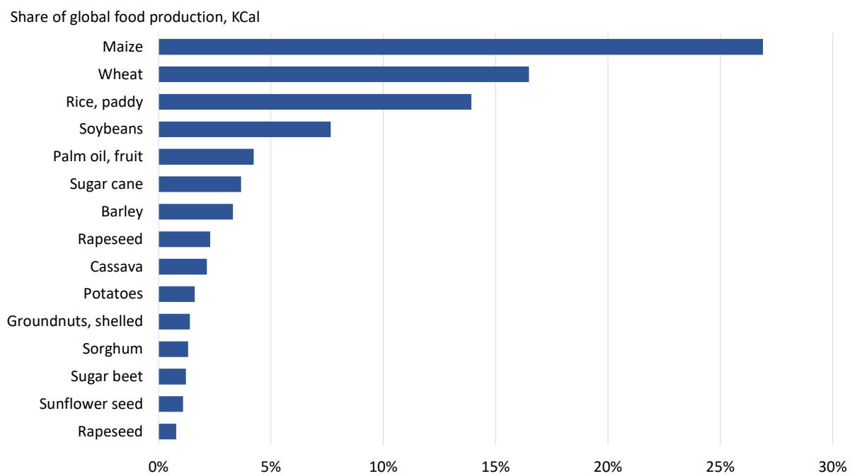
Figure 2 Global food production shares for selected commodities, 2019-21
