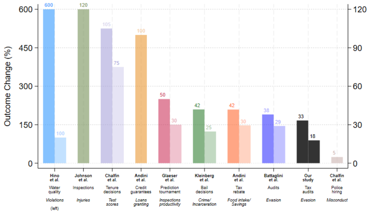
Figure G.1: Comparison of Optimized Results With Literature
