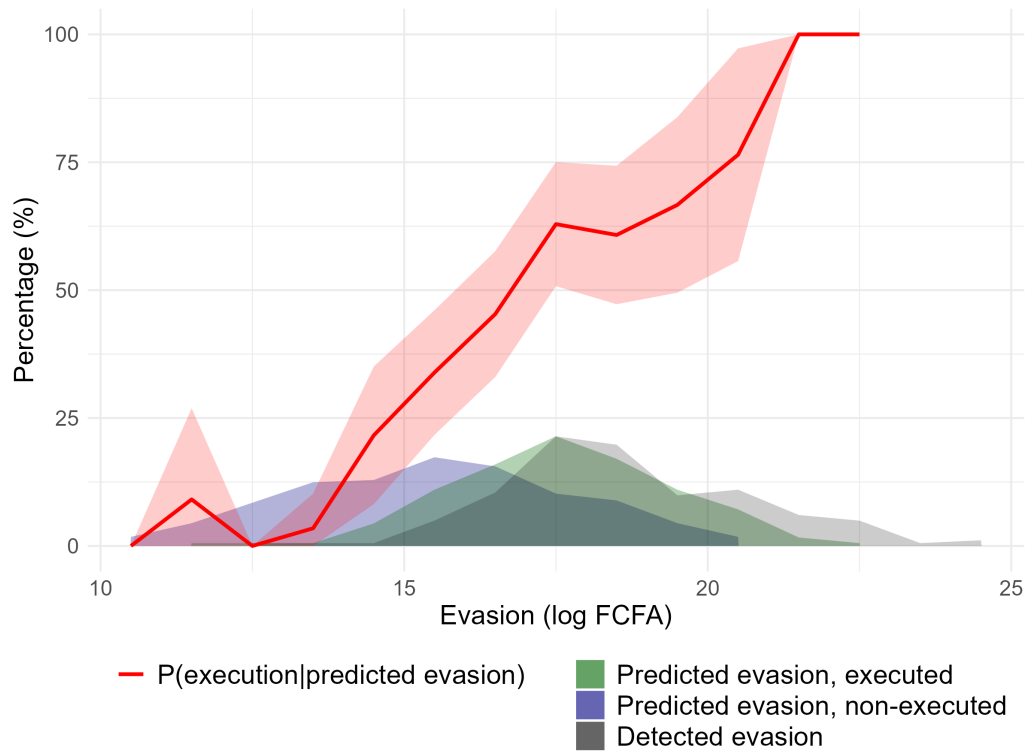
Figure F.3: Predicted and Realized Detected Evasion Amount
