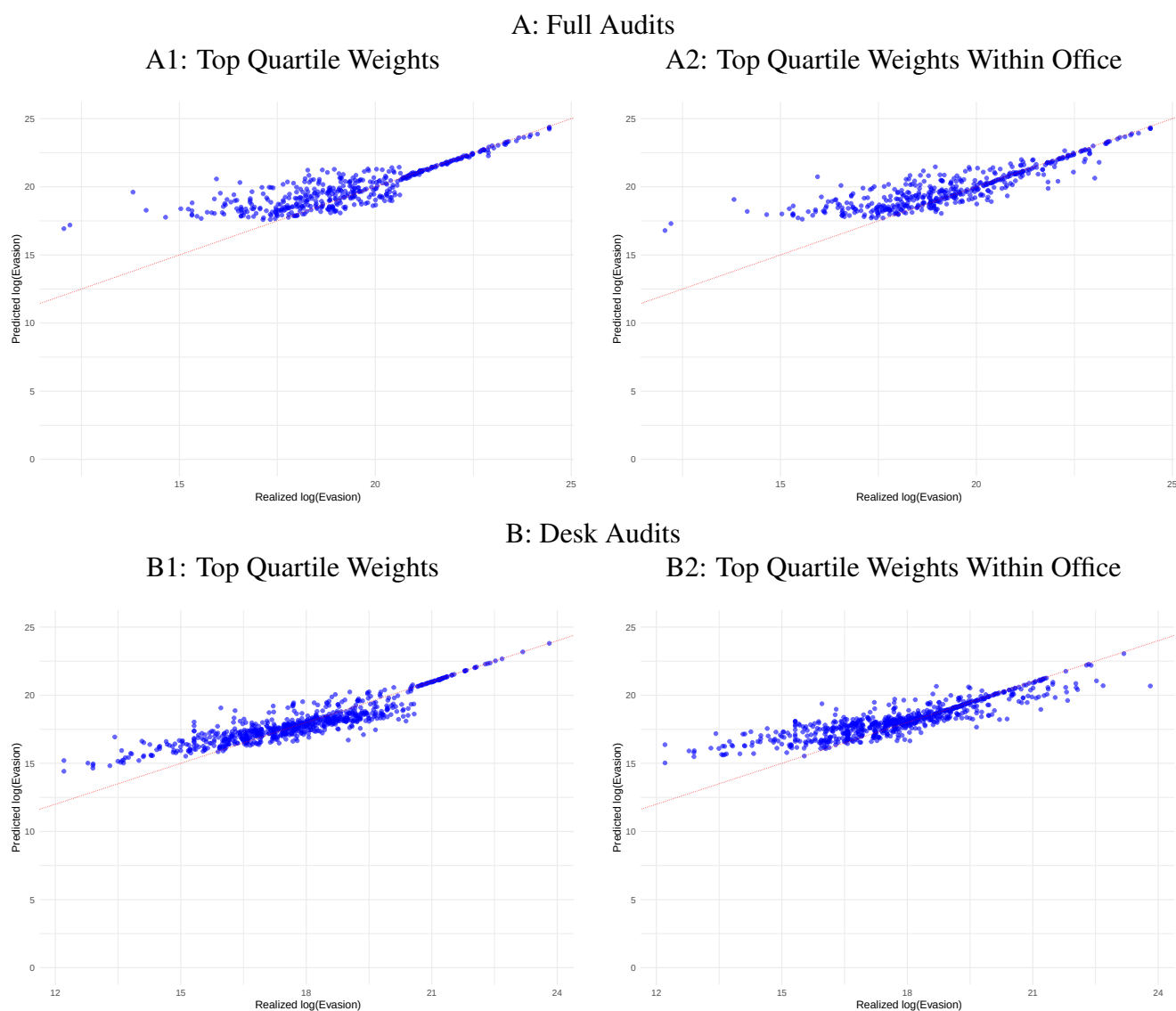
Figure G.2: Within-Sample Model Fit: Comparison of Predicted and Realized Evasion
