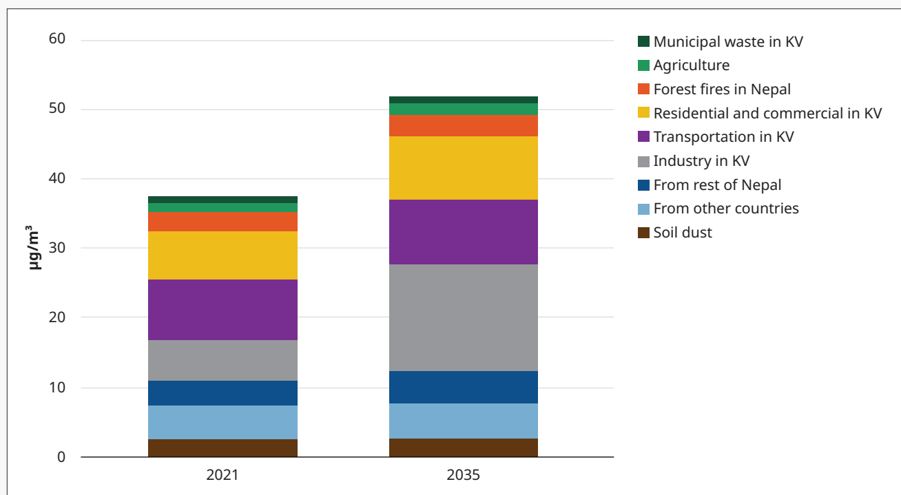
Figure 0.2: Population-weighted PM 2.5 annual average exposure in Kathmandu Valley, 2021-2035, by sector
