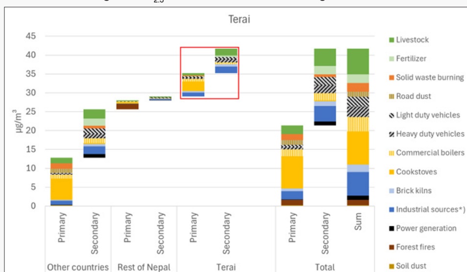
Figure D.19: Spatial and sectoral origin of PM_{2.5} in ambient air in the Terai region, 2021
