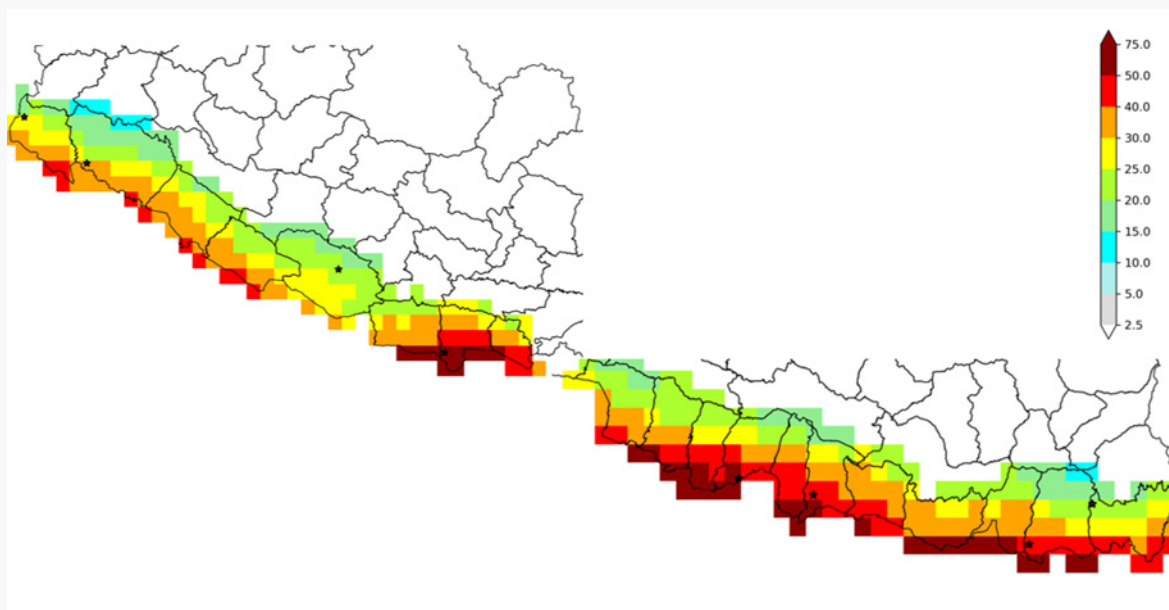
Figure D.6: Computed annual average concentrations of PM_{2.5} in the Terai ( \mu g/m^3 ), 2021
