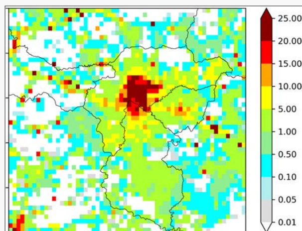
Figure D.3: Total primary PM 2.5 emissions in the Kathmandu Valley in 2021 (tons/cell)
