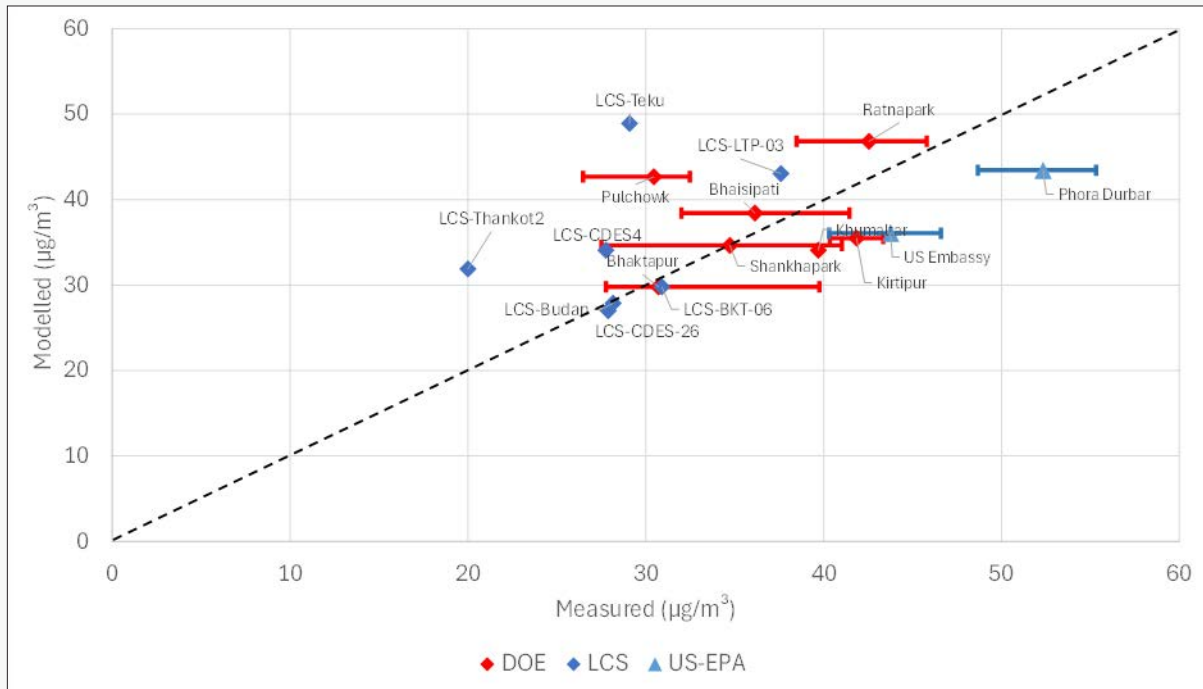
Figure D.12: Validation of estimated annual mean PM_{2.5} concentrations at specific locations in the Kathmandu Valley against modelled PM_{2.5} concentrations in the surrounding 1 km x 1 km grid cells.
