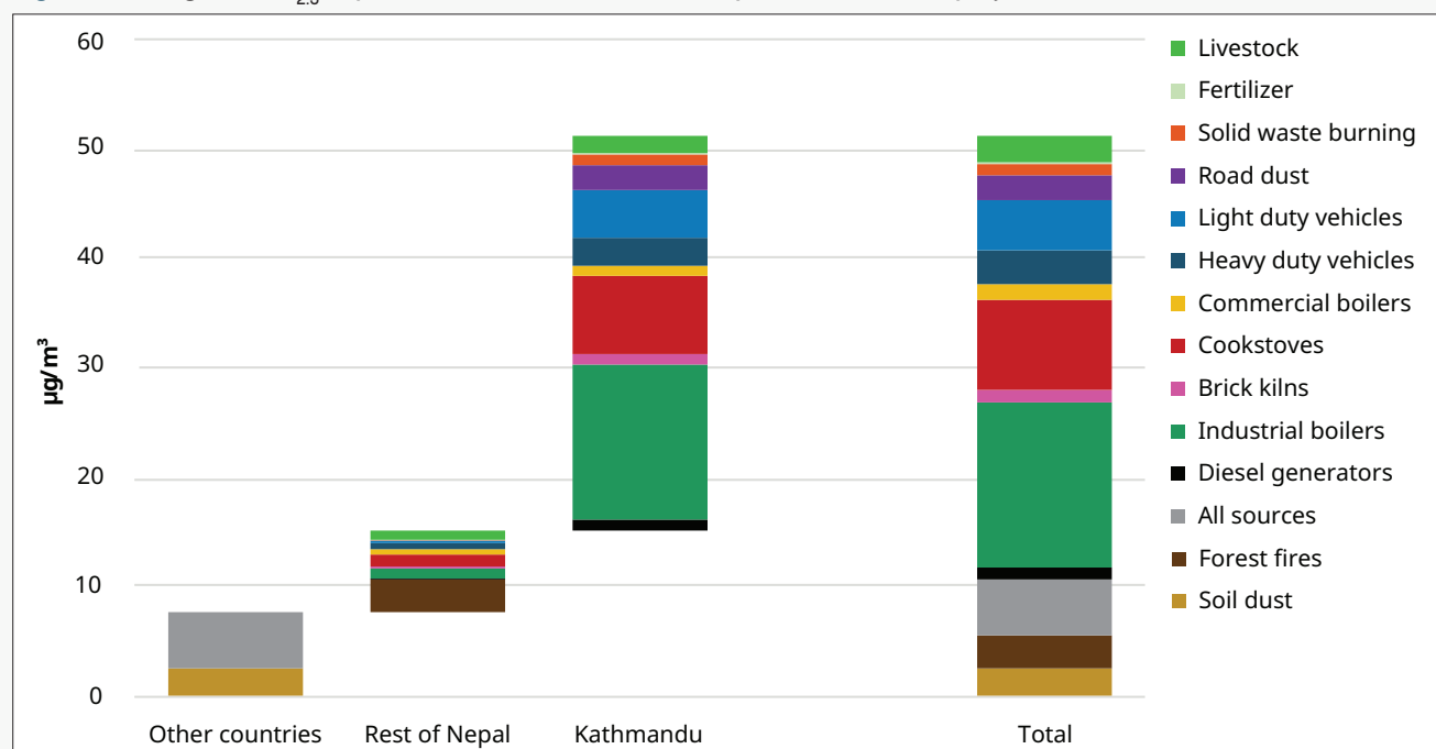
Figure 4.8: Origin of PM 2.5 exposure in the Kathmandu Valley for the baseline projection in 2035
