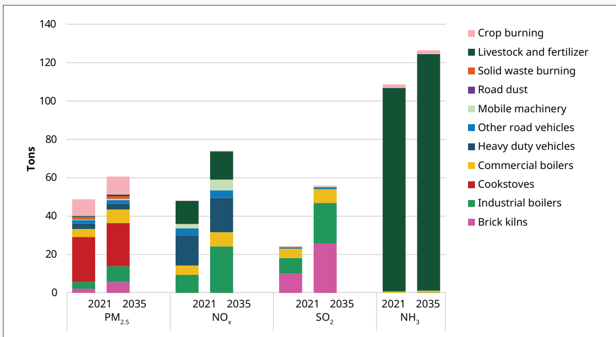
Figure 4.6: Baseline emissions in the Terai, 2021-2035, by sector
