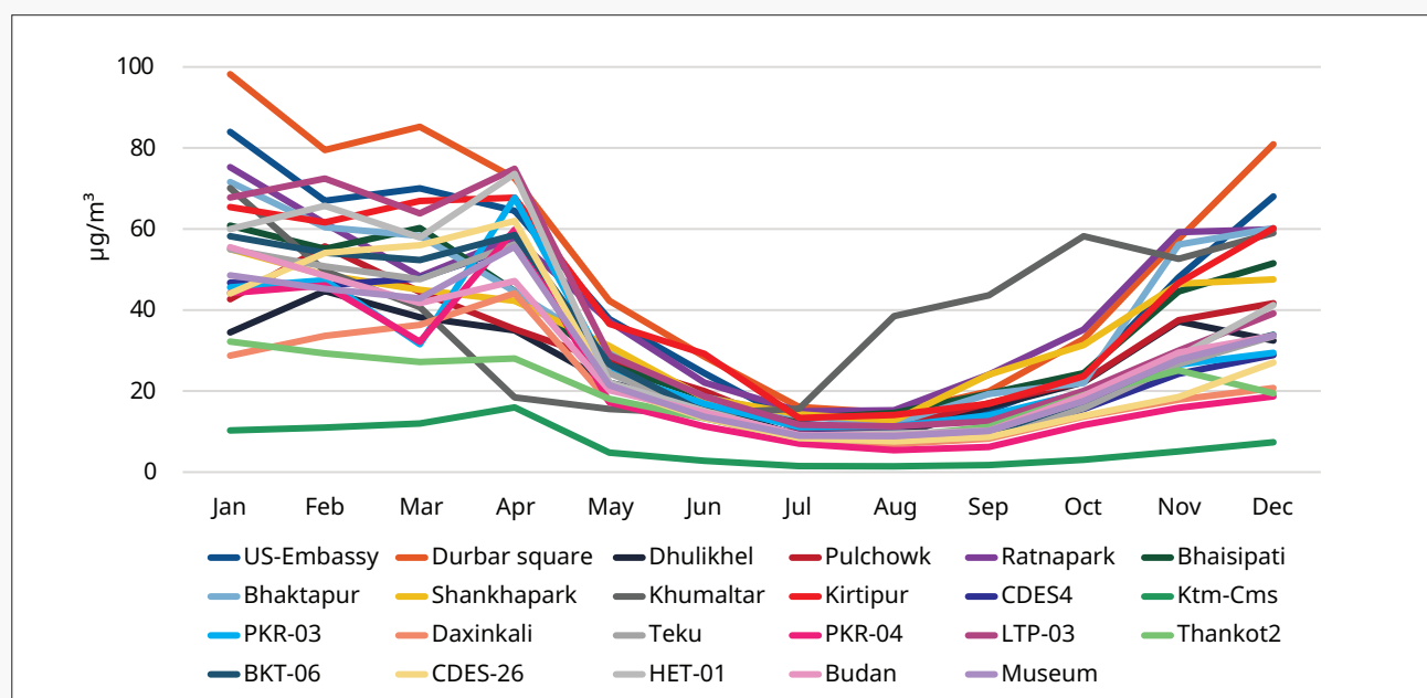
Figure 1.4: Monthly trends of PM 2.5 in the Kathmandu Valley (monthly average concentrations of the years with available data)
