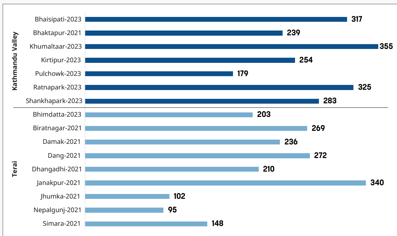
Figure 1.7: Total days of PM 2.5 data availability in 2021 and 2023
