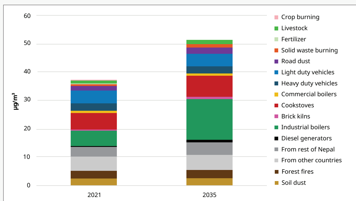
Figure 4.7: Population weighted PM 2.5 exposure in the Kathmandu Valley, 2021-2035, by sector
