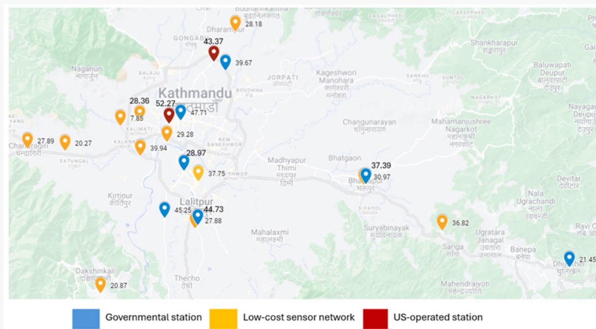
Figure D.8: Locations of the monitoring stations with sufficient data coverage in the Kathmandu Valley. Figures refer to recent measurements of annual average \text{PM}_{2.5} concentrations ( \mu\text{g}/\text{m}^3 )
