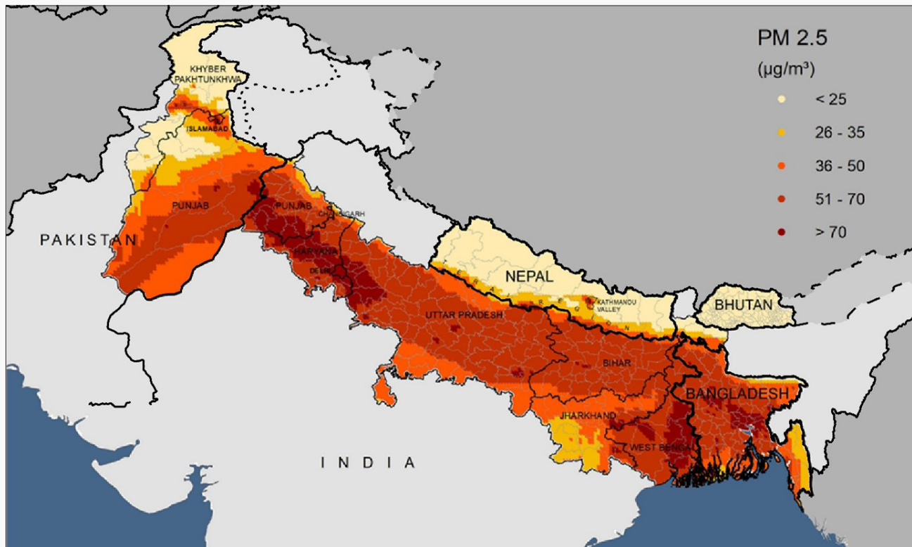
Figure 0.3: Air pollution concentrations in Nepal and the other four countries sharing the Indo-Gangetic Plain and Himalayan Foothills (IGP-HF) airshed, 2021
