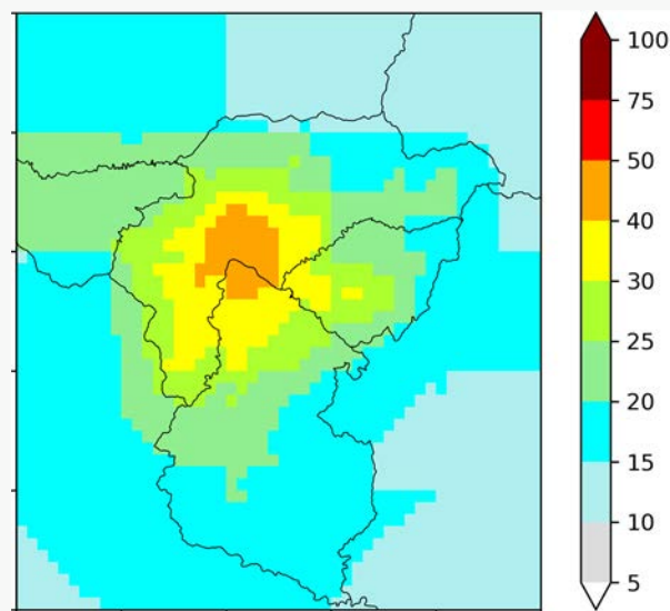
Figure D.5: Computed annual average concentrations of PM 2.5 in the Kathmandu Valley (µg/m 3 ), 2021
