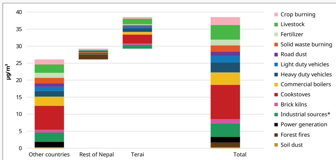
Figure 4.4: Spatial and sectoral origin of PM 2.5 in ambient air in the Terai region, 2021
