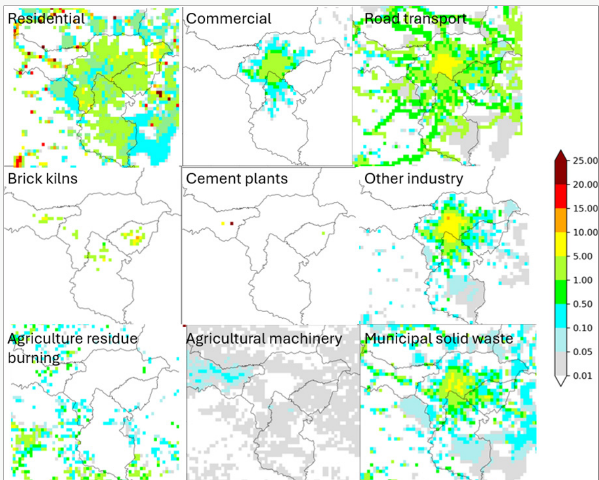
Figure D.2: Primary emissions of PM_{2.5} from the various source sectors in the Kathmandu Valley in 2021 (tons/cell)
