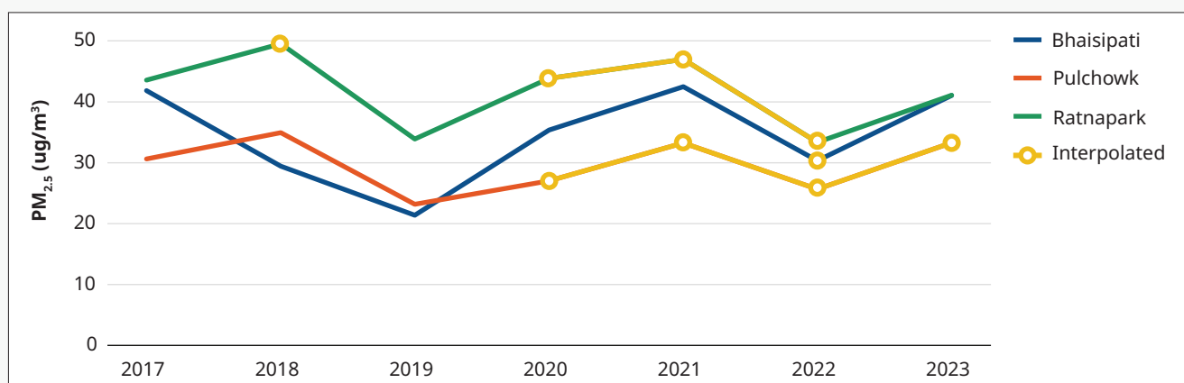
Figure 1.3: Annual average PM 2.5 (µg/m 3 ) concentration trends in the Kathmandu Valley (2017-2023)
