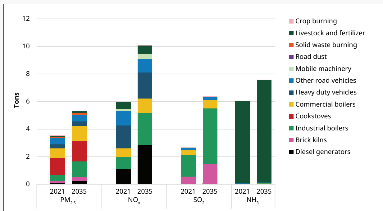
Figure 4.5: Baseline emissions in the Kathmandu Valley, 2021-2035, by sector
