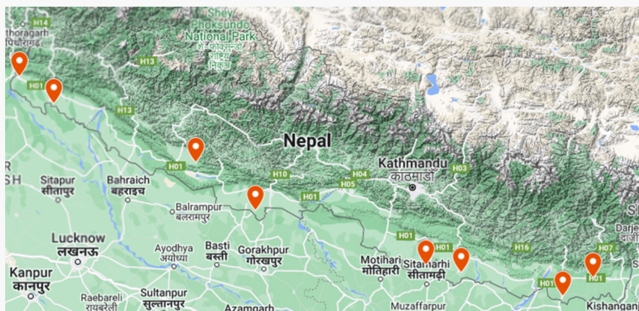
Figure D.10: Locations of the monitoring stations with sufficient data coverage in the Terai
