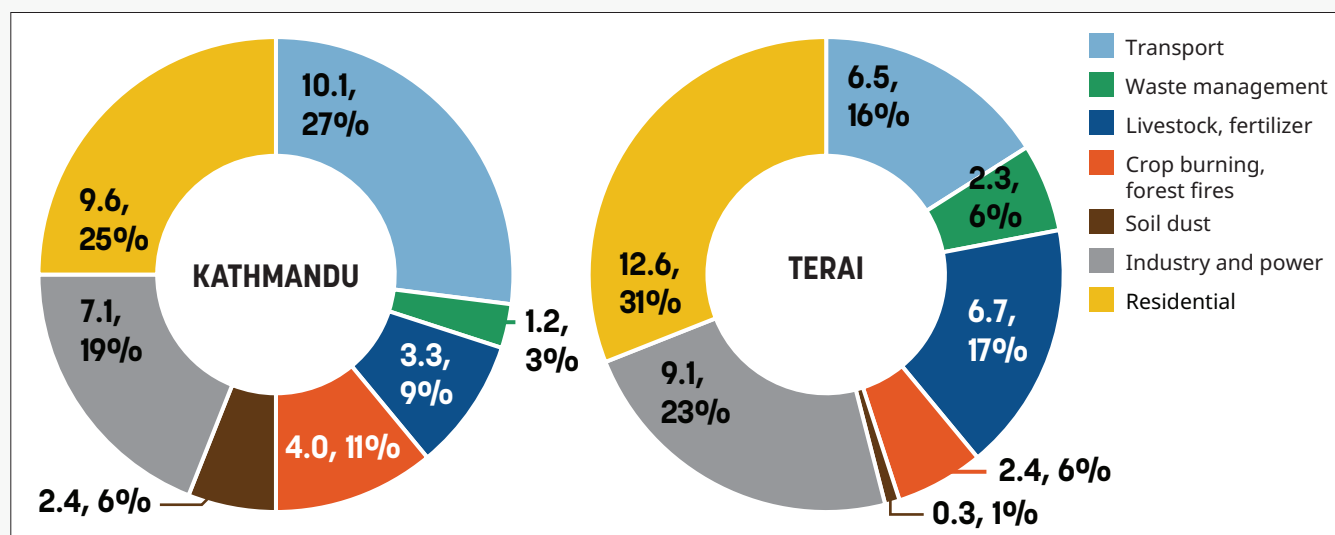
Figure 4.1: Contributions of different source sectors to population-weighted annual-average PM_{2.5} concentrations in the Kathmandu and the Terai in 2021 (in \mu g/m^3 and %)
