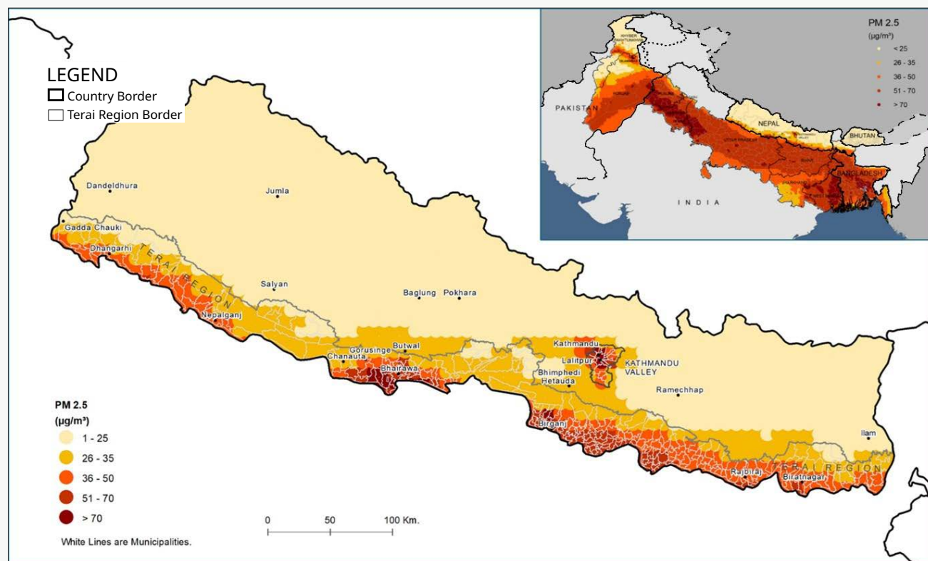
Figure 1.1: PM 2.5 concentrations ( \mu\text{g}/\text{m}^3 ) in Nepal and other four countries sharing the Indo-Gangetic Plain and Himalayan Foothills (IGP-HF) region, 2021
