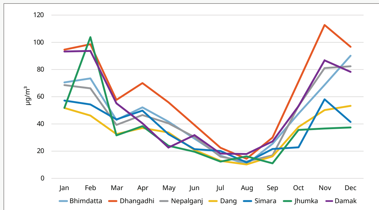
Figure 1.5: Monthly trends of PM 2.5 in the Terai (monthly average concentrations of the years with available data)
