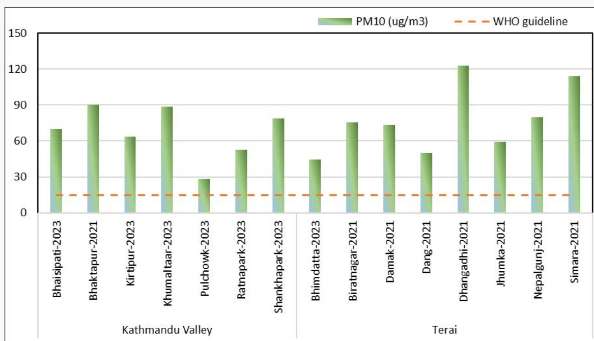
Figure A.4: Annual average PM 10 for the Kathmandu Valley and the Terai, for the period 2021 and 2023
