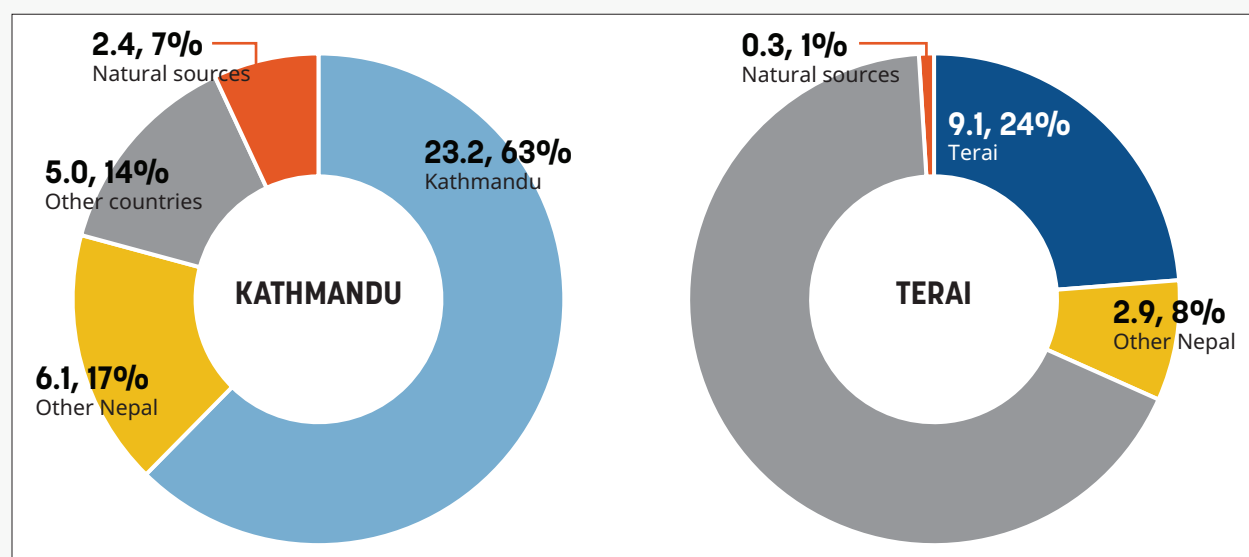
Figure 4.2: Spatial origin of PM 2.5 in ambient air in the Kathmandu and the Terai in 2021 (in µg/m 3 and %)
