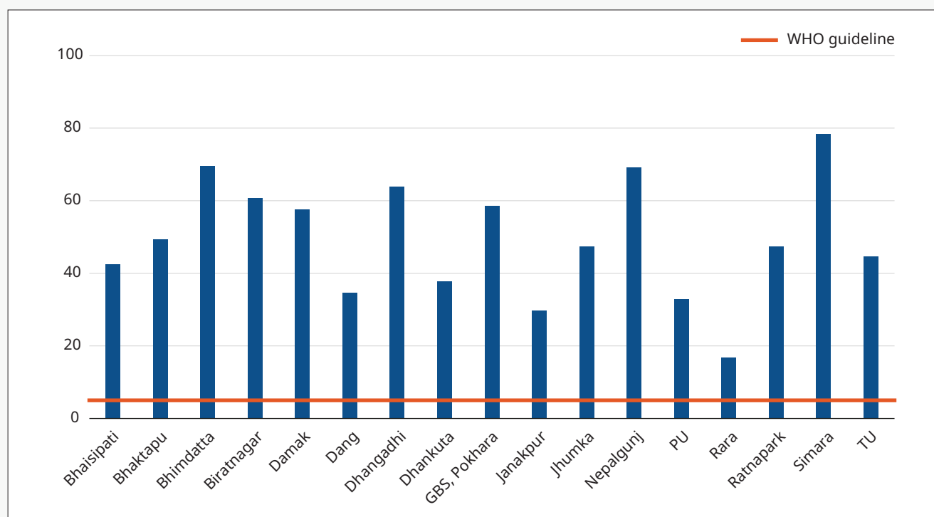
Figure 1.2: Annual average PM 2.5 concentrations in the Kathmandu Valley and the Terai region, by monitored locations
