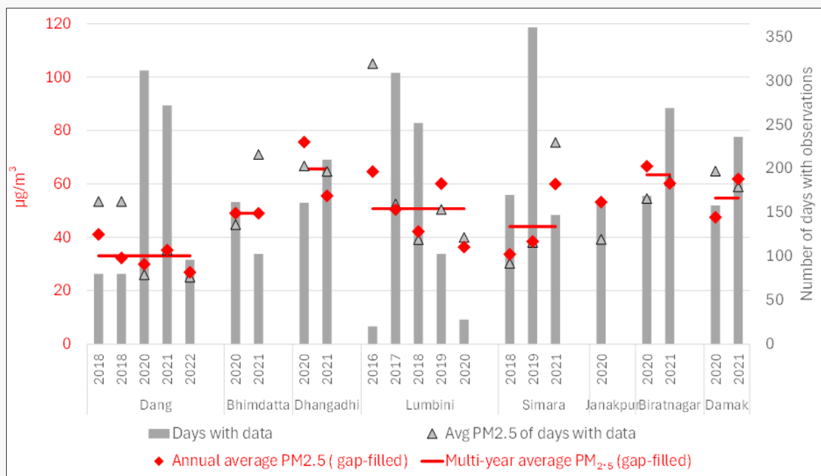
Figure D.11: Annual average concentrations of PM_{2.5} measured at monitoring stations in the Terai
