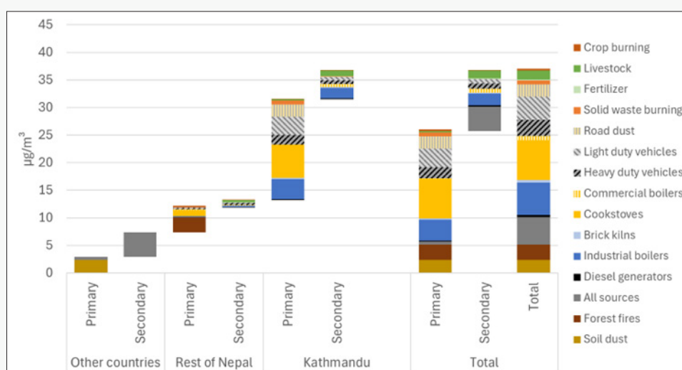
Figure D.18: Spatial and sectoral origin of PM_{2.5} in ambient air in the Kathmandu Valley, 2021
