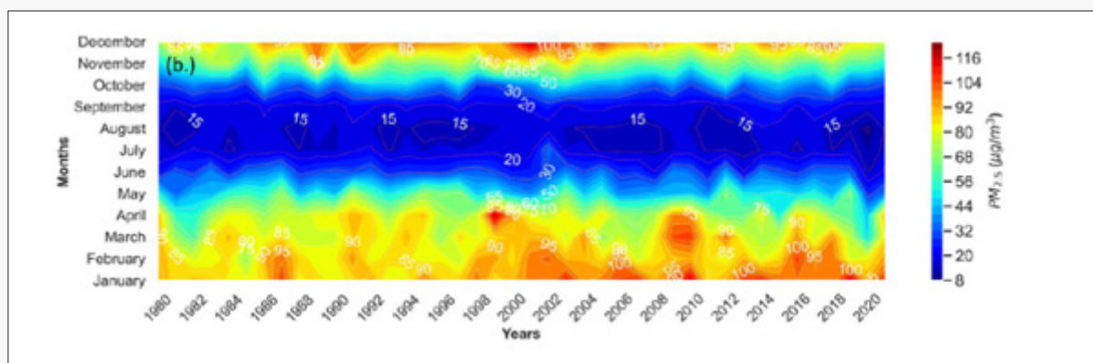
Figure A.2: Monthly average PM_{2.5} for the Kathmandu, reconstructed for the period 1980 to 2021
