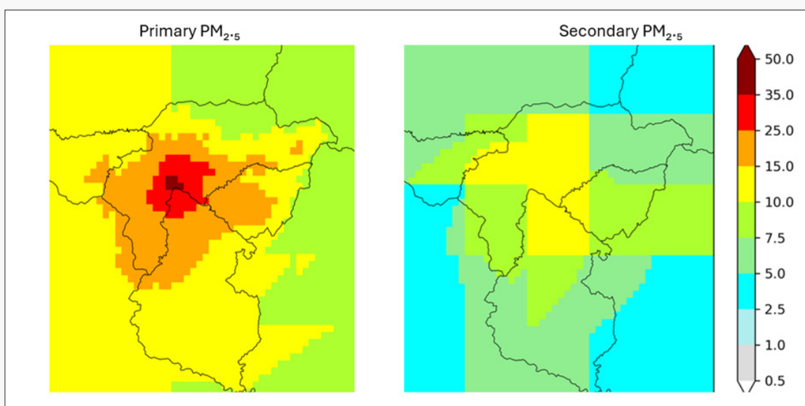
Figure D.15: Annual mean concentrations of primary and secondary \text{PM}_{2.5} in Kathmandu 2021 ( \mu\text{g}/\text{m}^3 )
