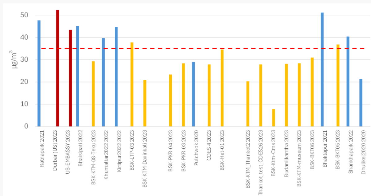
Figure D.9: Annual average concentrations of PM 2.5 measured at monitoring stations in the Kathmandu Valley
