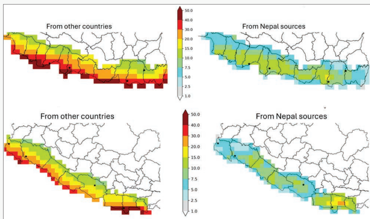
Figure D.16: The spatial origin of \text{PM}_{2.5} concentrations in the Terai East (upper panel) and the Terai West (lower panel) in 2021 ( \mu\text{g}/\text{m}^3 )
