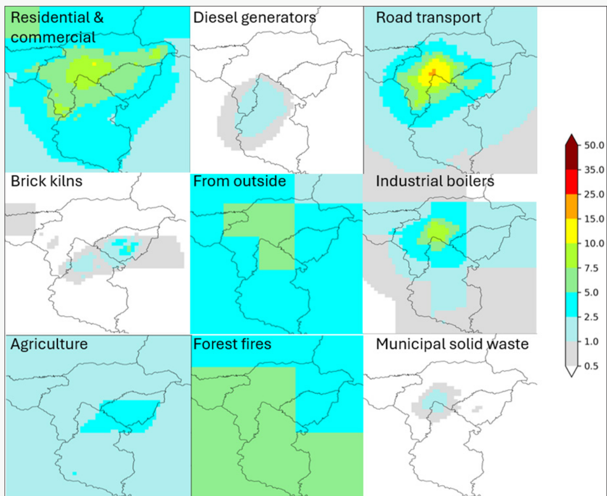
Figure D.14: Contributions of the various emission source sectors to annual mean PM 2.5 concentrations in the Kathmandu Valley in 2021 (µg/m 3 )
