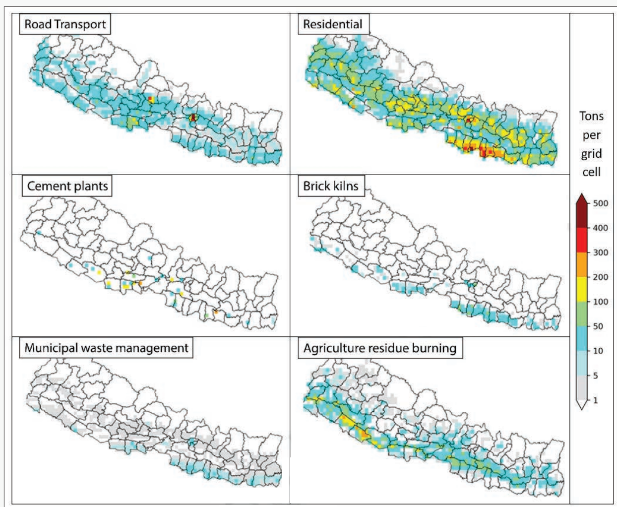
Figure D.4: Density of primary PM 2.5 emissions from the various sectors in Nepal, 2021
