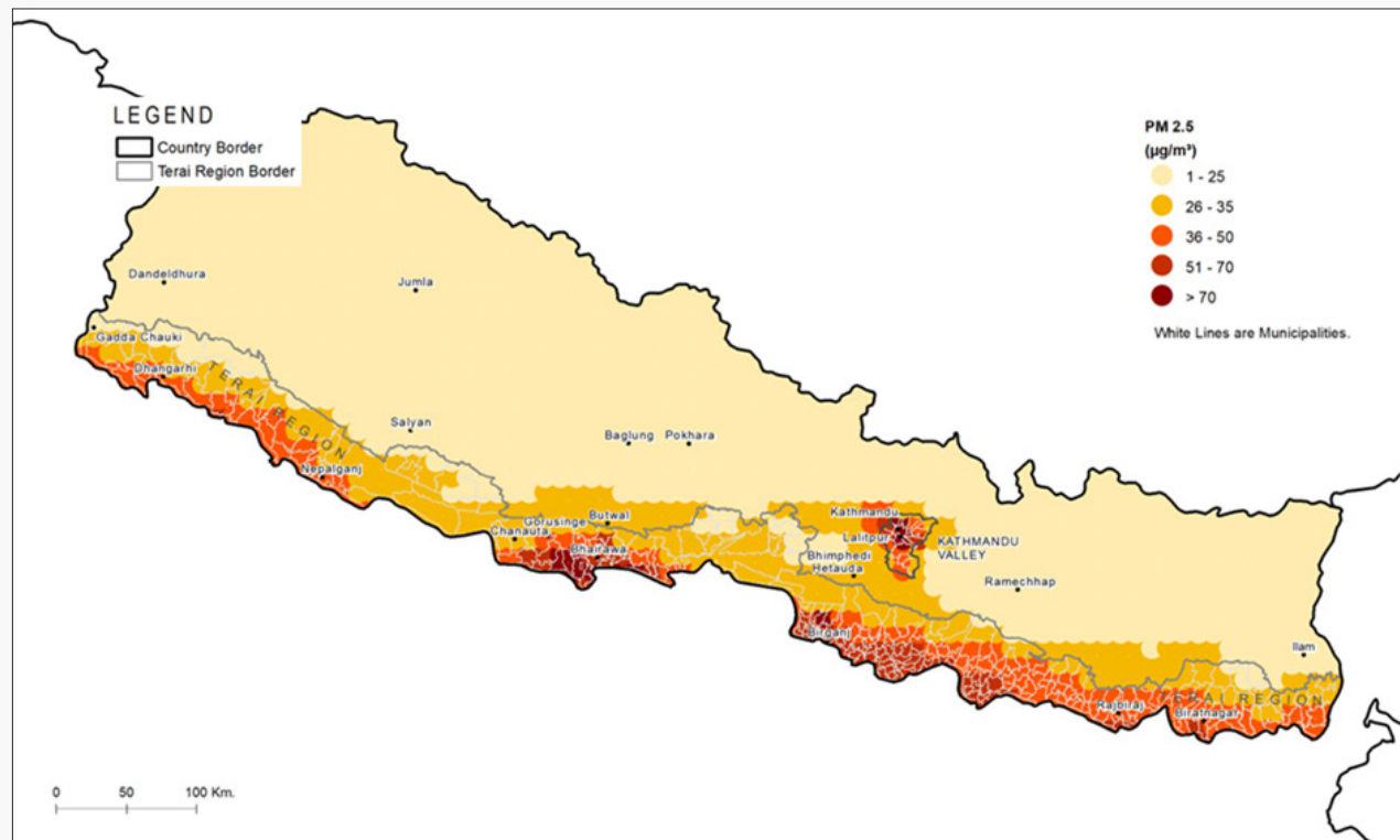
Figure 0.1: Average annual air pollution concentrations in Nepal, 2021
