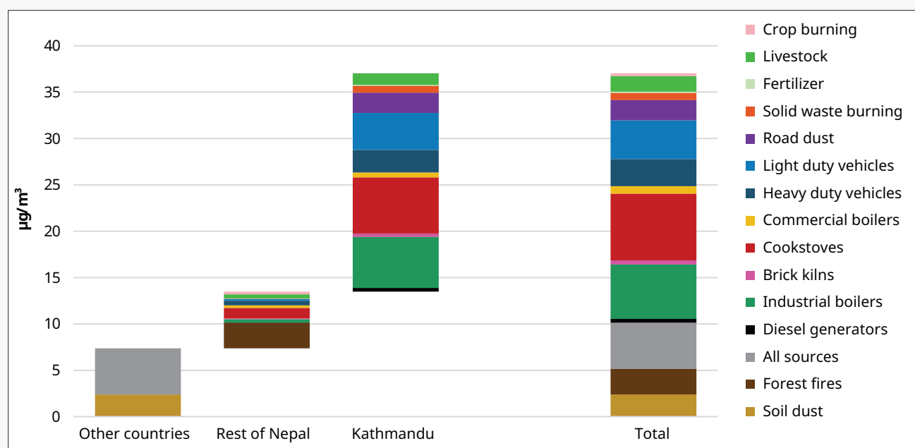
Figure 4.3: Spatial and sectoral origin of PM_{2.5} in ambient air in the Kathmandu Valley, 2021
