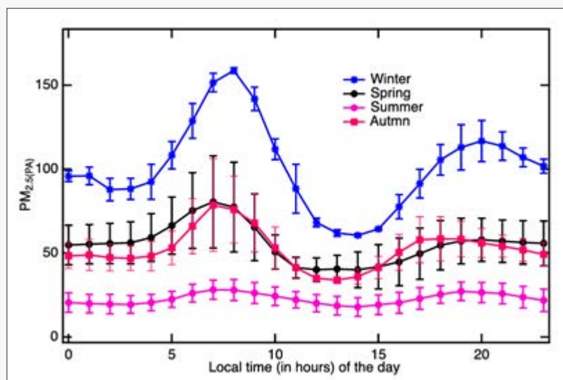
Figure A.1: Diurnal cycle of PM 2.5 in Pulchowk, Kathmandu Valley, for each season
