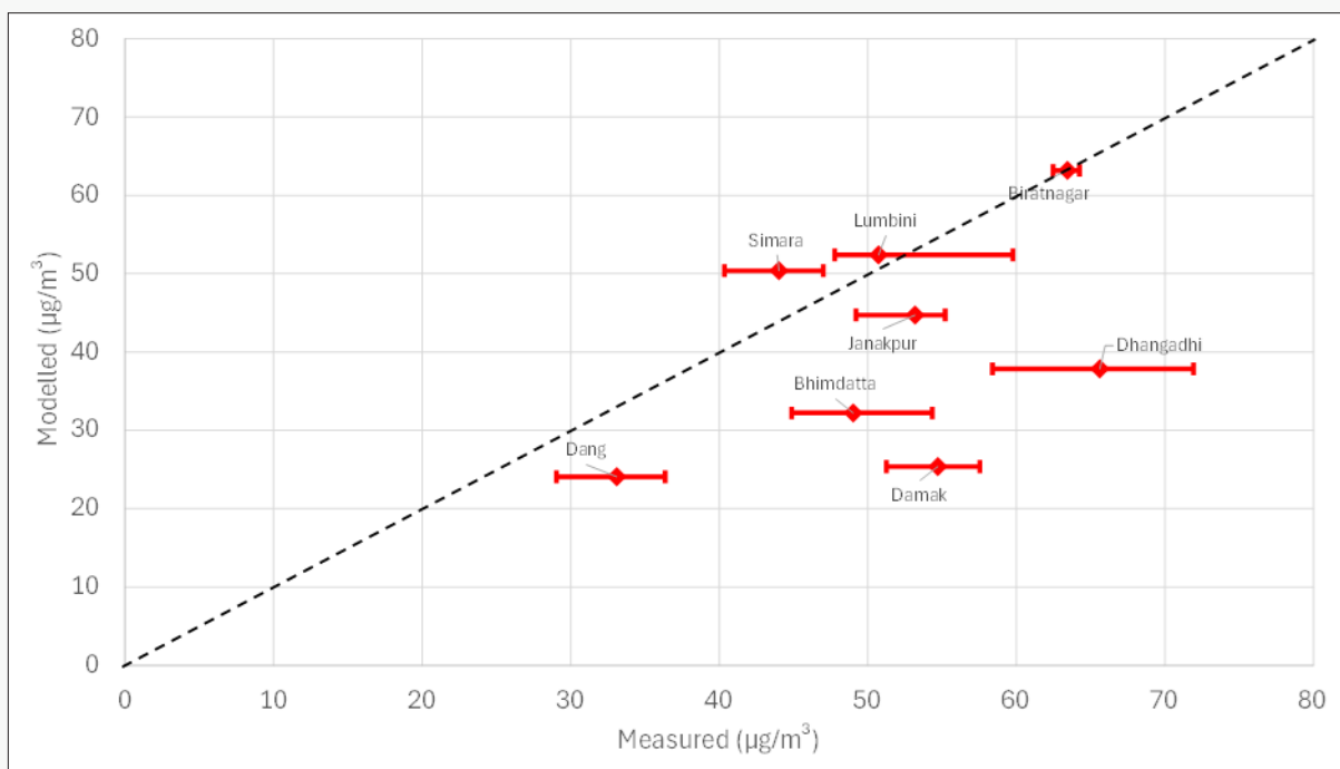
Figure D.13: Validation of estimated annual mean PM_{2.5} concentrations at specific locations in the Terai against modelled PM_{2.5} concentrations in the surrounding 1 km x 1 km grid cells.
