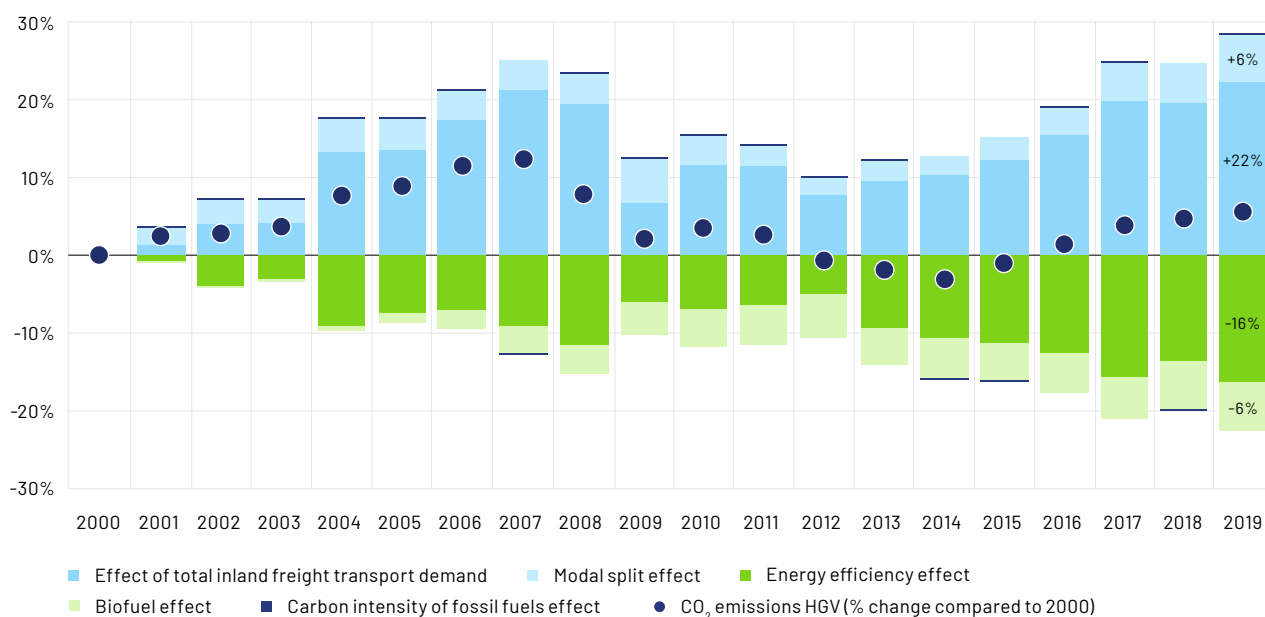
Figure 2.5. Decomposition Analysis of direct (tailpipe) CO 2 Emissions from Trucks in the EU (2000–19)
