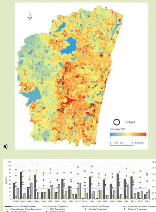
Figure 2-8. a) UHI index and the 100 spots selected across CMA; b) air temperature (field survey data) variation with the urban morphology indices and other metadata sources, mapped across the 20 spots in CMA. Source: World Bank n.d.
