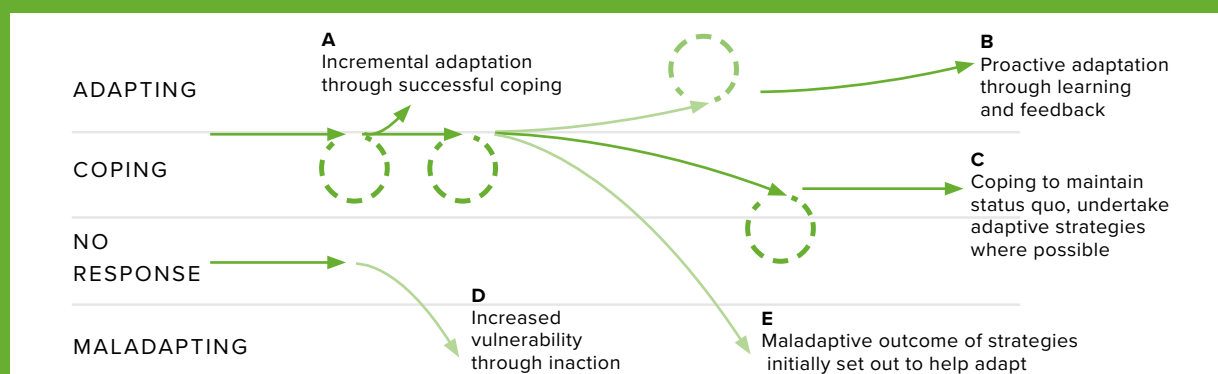
Figure 2-15. Conceptual diagram of adaptation outcomes over time, including maladaptation Source: Schipper 2020.
