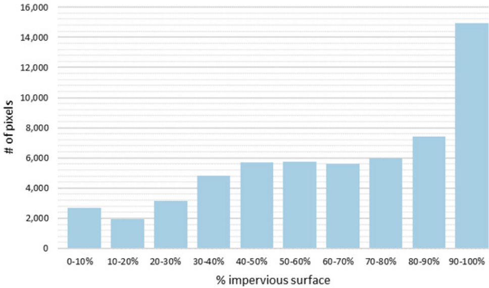
Figure B.5. Distribution of Pixels in the Area of Analysis in Terms of Impervious Cover
